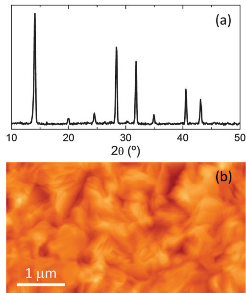
Fig. 2 (a) GIXRD pattern and (b) AFM topography of a \text{CH}_3\text{NH}_3\text{PbI}_3 thin film deposited by flash evaporation.
